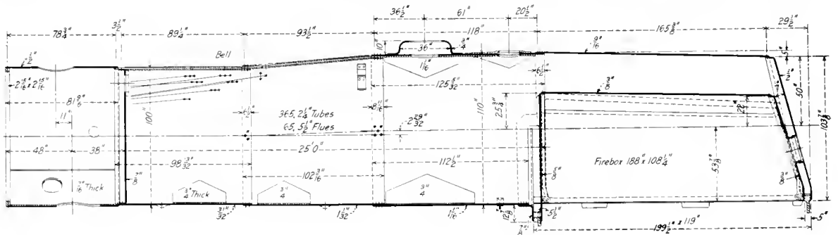
Boiler of the Virginian Triplex Locomotive
